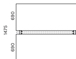
LAUAPLAADID / DESK TOPS PAPLK14069 / 1400x1475 PAPLK16069 / 1600x1475 PAPLK18069 / 1800x1475
